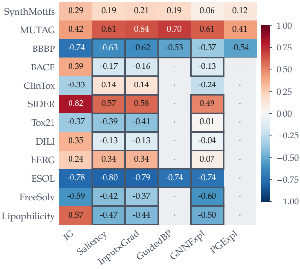
occlusion faithfulness (Spearman \rho )
