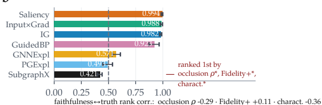
b MolMotifHard-GINE: in-distribution, n=200
