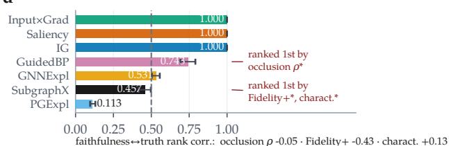
d Benzene-GINE: in-distribution, n=200
