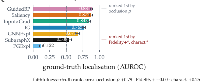
e FluorideCarbonyl-GINE: in-distribution, n=200
