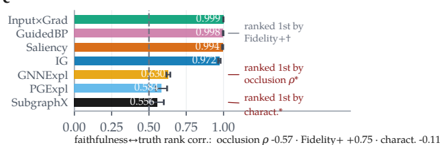
c MolMotif-GINE: in-distribution, n=200
