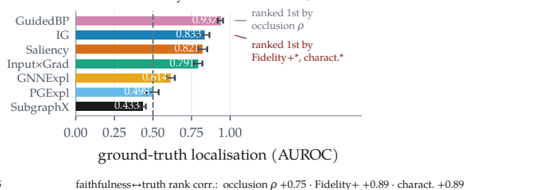
FluorideCarbonyl-GINE: scaffold shift, n=200
