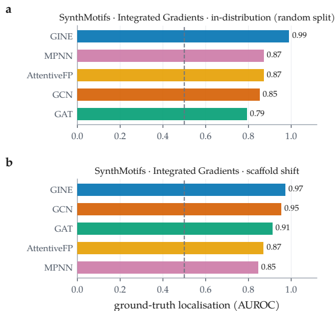
Figure 7: The backbone ordering does not survive the change of split. Integrated Gradients held fixed; ground-truth localisation across the 5 backbones on SynthMotifs, in distribution (a) and under scaffold shift (b). Dashed line is chance. Spearman correlation between the two orderings is 0.100 over 5 backbones.
