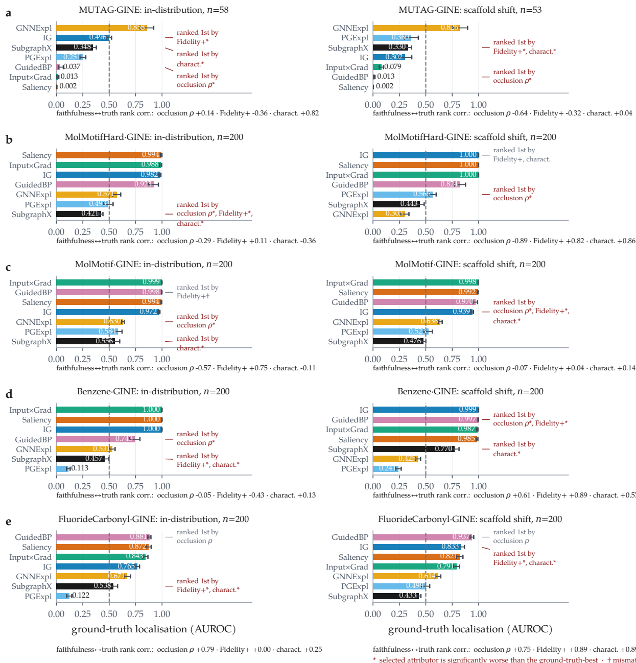
Figure 5: A faithfulness-only ranking selects the wrong attributor in 26 of 30 tests, in distribution as well as under shift. Ground-truth localisation per attributor, with bootstrap 95% confidence intervals over molecules. Within each row the dataset, backbone and attributor set are fixed and only the split changes; significant picks are marked *, picks statistically indistinguishable from the best are marked †. Rows, top to bottom: MUTAG (motif-proxy ground truth), where all 3 metrics mismatch in both regimes and under shift the occlusion measure selects GuidedBP, whose localisation (0.013) is anti-aligned with the motif; MolMotifHard and MolMotif (real molecules, exact node ground truth by construction), where the label is the substructure; and Benzene and FluorideCarbonyl , the Sanchez-Lengeling et al. [9] rationale benchmarks, whose per-atom labels we did not author. The mismatch is near-universal; what varies across rows is its cost, from 0.002 to 0.821 AUROC. Rank correlations between each faithfulness metric and ground truth are given below each panel.
