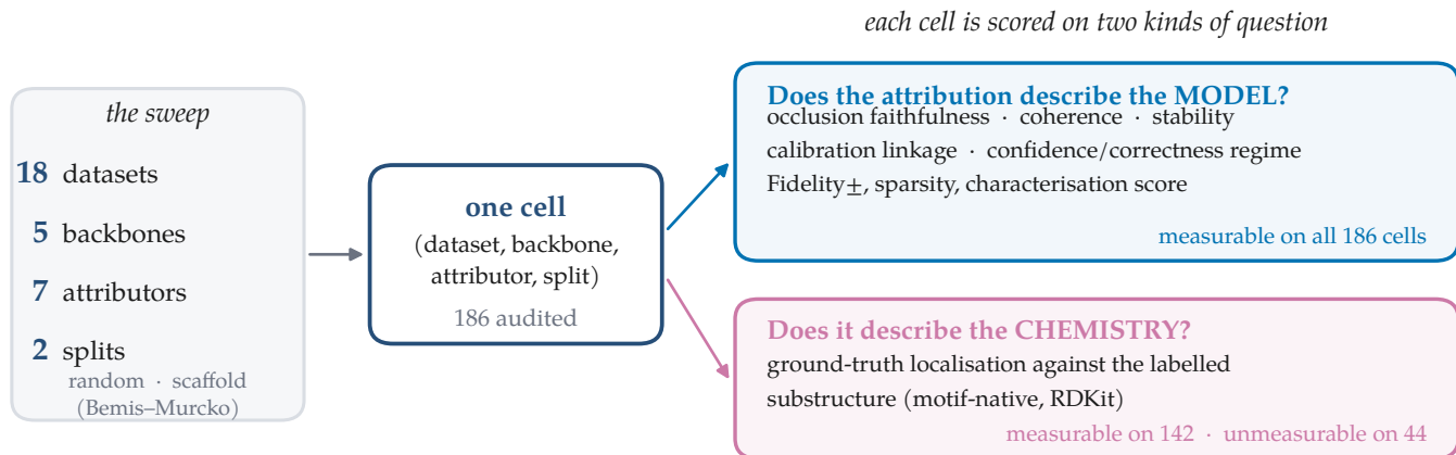
Figure 1: What the audit does, and the asymmetry it is built around. The sweep produces one cell — a (dataset, backbone, attributor, split) combination — as the unit of every claim in this paper. Each cell is scored on axes that ask whether the attribution describes the model , which are computable wherever an attribution is, and on one axis that asks whether it describes the chemistry , which needs per-atom labels and is therefore unavailable on every real molecular property dataset in the sweep. An evaluation framework that reports only the first column rates a cell in the lower-right of Figure 3 — faithful to the model, anti-aligned with the truth — as fine. Counts are read from the committed results, not annotated by hand.
