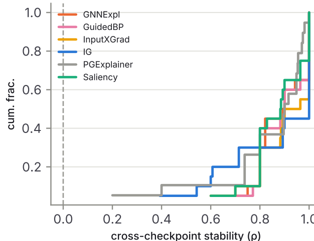
e MUTAG · stability
