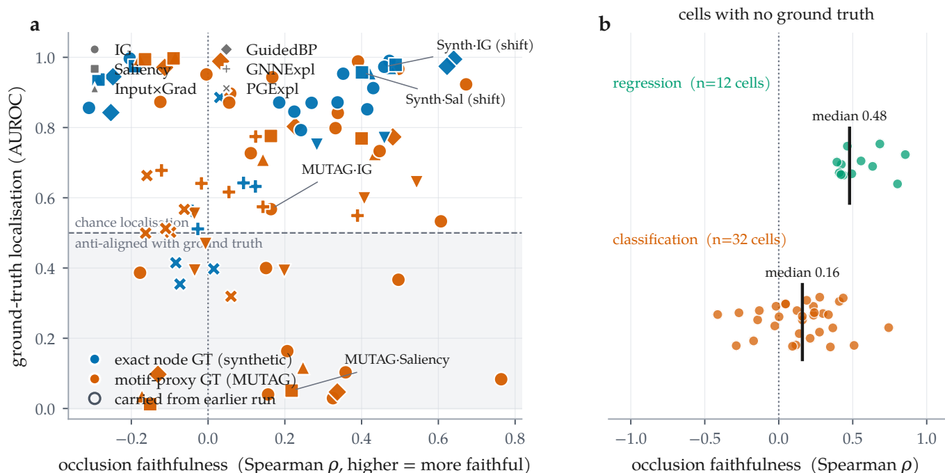
Figure 1: The two axes come apart, and for most cells only one of them exists. (a) Every committed cell carrying a node-level ground truth ( n = 92 ), plotted as occlusion faithfulness against ground-truth localisation; colour distinguishes exact synthetic ground truth from the MUTAG motif proxy, marker distinguishes attributor, and open markers are rows carried from an earlier run. The shaded band is GT AUROC < 0.5 : attributions there are anti-aligned with the true motif. 13 cells sit in the lower-right region, positively faithful to the model and anti-aligned with the truth. (b) The remaining 44 combinations, on real molecular datasets, have no published per-atom labels: only the horizontal axis is measurable for them.
