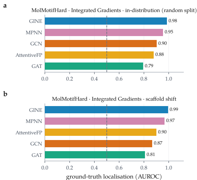
Figure 7: Which backbone localises best is a large effect, and a stable one across the split. Integrated Gradients held fixed; ground-truth localisation across the 5 backbones on MolMotifHard — a molecular arm with exact node labels, so its scaffold split is a chemical regime — in distribution (a) and under scaffold shift (b). Dashed line is chance. The two orderings correlate at \rho = 0.900 over 5 backbones, and at 0.700–0.900 across the 3 molecular arms carrying the full sweep. The gap between best and worst backbone is 0.191 AUROC in distribution and 0.186 under shift: the architecture matters, and it matters the same way in both regimes.
