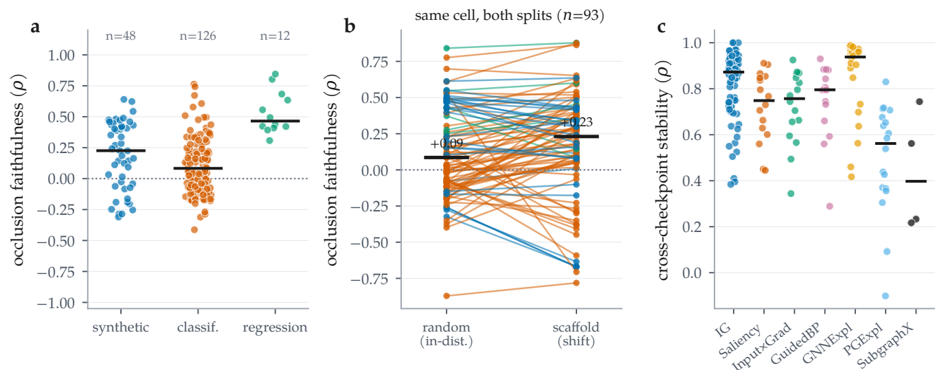
Figure 9: Distributions across all audited combinations. (a) Occlusion faithfulness by dataset regime; bars are medians. (b) The same cell on both splits, joined: faithfulness falls under the scaffold split in only 36 of 93 cells (median change 0.077), so shift does not systematically reduce faithfulness. (c) Cross-checkpoint stability by attributor; the mask-learning methods are not uniformly more stable than the gradient ones.
