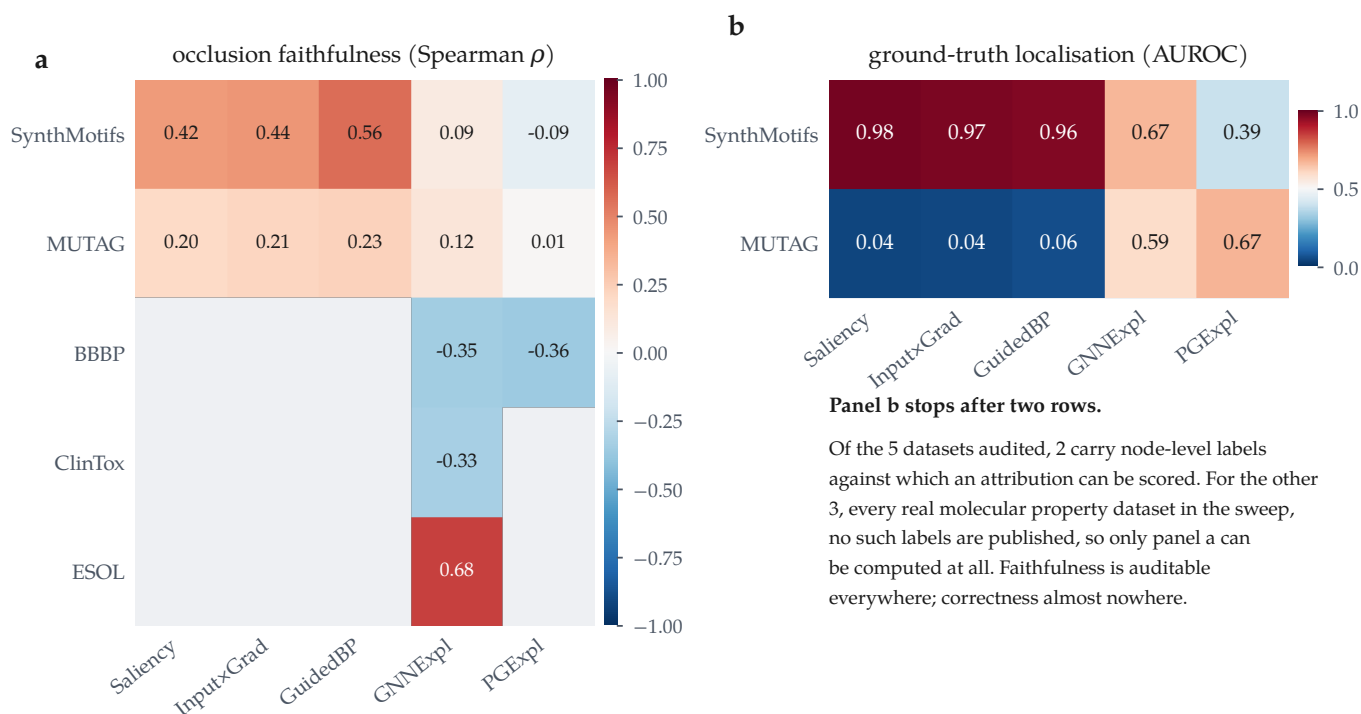
Figure 4: Reliability is a property of the (attributor, dataset) pair, not of the attributor. All committed GINE cells at the scaffold split. (a) Occlusion faithfulness over every audited dataset; blue = anti-faithful. (b) Ground-truth localisation, which exists for two datasets only. Panel b is short because correctness is unmeasurable elsewhere, not because it scores badly there: no molecular dataset in the sweep publishes per-atom labels. Blank cells were not audited; a thin outline marks a value carried from an earlier run.
