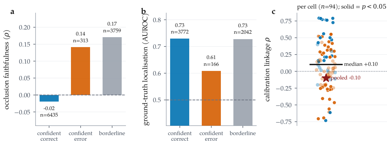
Figure 6: Regime stratification and calibration linkage, over the 12113 per-molecule audit records. (a) Occlusion faithfulness and (b) ground-truth localisation by confidence/correctness regime; n is printed per bar because ground truth exists for only a minority of molecules. Localisation on confident-error molecules falls below chance (0.608, n = 166 ) while occlusion faithfulness on the same molecules is unremarkable. (c) Calibration linkage computed per cell (solid = p < 0.05 ): the median cell is positive, but pooling all molecules into one correlation reverses the sign, a Simpson’s paradox and a caution against reporting the pooled number.
