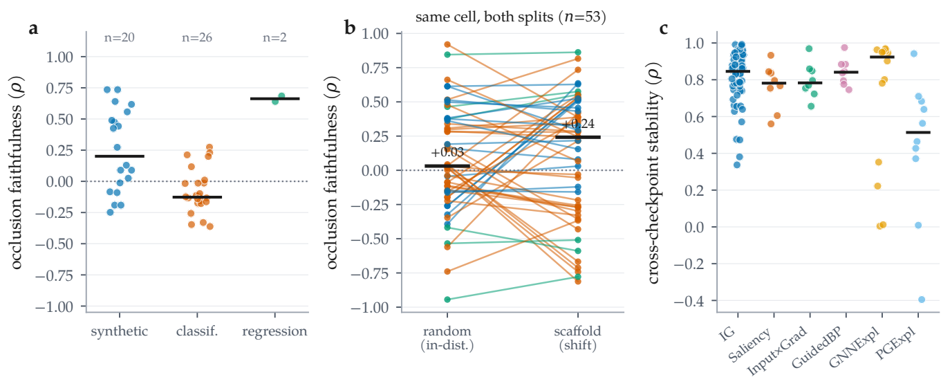
Figure 5: Distributions across all audited combinations. (a) Occlusion faithfulness by dataset regime; bars are medians. (b) The same cell on both splits, joined: faithfulness falls under the scaffold split in only 28 of 53 cells (median change -0.009 ), so shift does not systematically reduce faithfulness. (c) Cross-checkpoint stability by attributor; the mask-learning methods are not uniformly more stable than the gradient ones.
