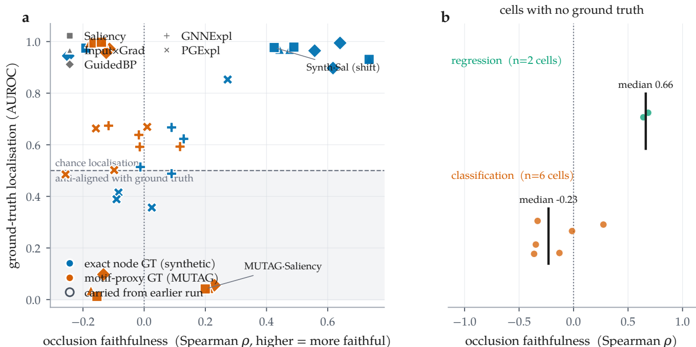
Figure 1: The two axes come apart, and for most cells only one of them exists. (a) Every committed cell carrying a node-level ground truth ( n = 40 ), plotted as occlusion faithfulness against ground-truth localisation; colour distinguishes exact synthetic ground truth from the MUTAG motif proxy, marker distinguishes attributor, and open markers are rows carried from an earlier run. The shaded band is GT AUROC < 0.5 : attributions there are anti-aligned with the true motif. 5 cells sit in the lower-right region, positively faithful to the model and anti-aligned with the truth. (b) The remaining 8 combinations, on real molecular datasets, have no published per-atom labels: only the horizontal axis is measurable for them.
