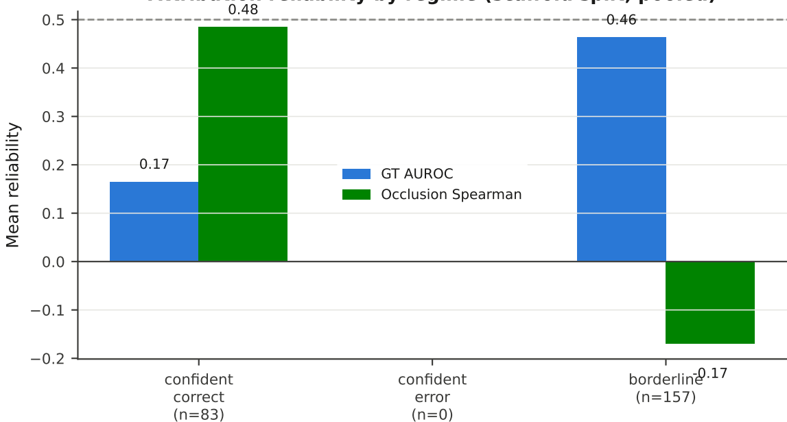
Attribution reliability by regime (scaffold split, pooled)
