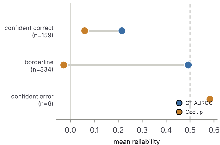
f reliability by regime (pooled)
