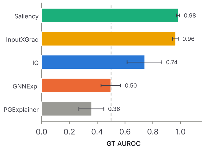
b SynthMotifs (exact GT) · by attributor
