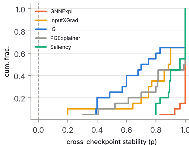
e MUTAG · stability
