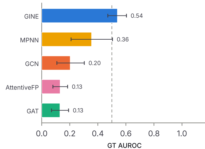
c MUTAG · IG · by backbone
