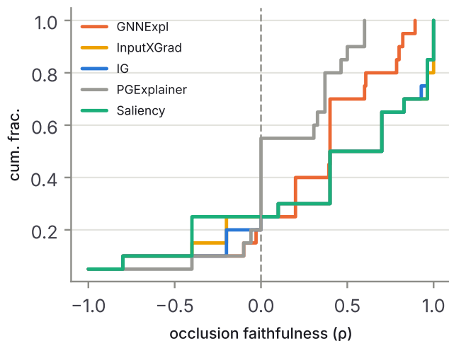
d MUTAG · faithfulness
