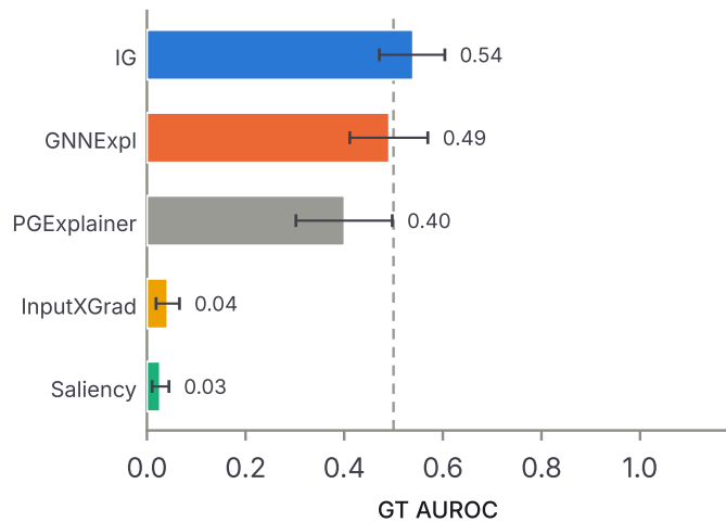
a MUTAG (proxy GT) · by attributor
