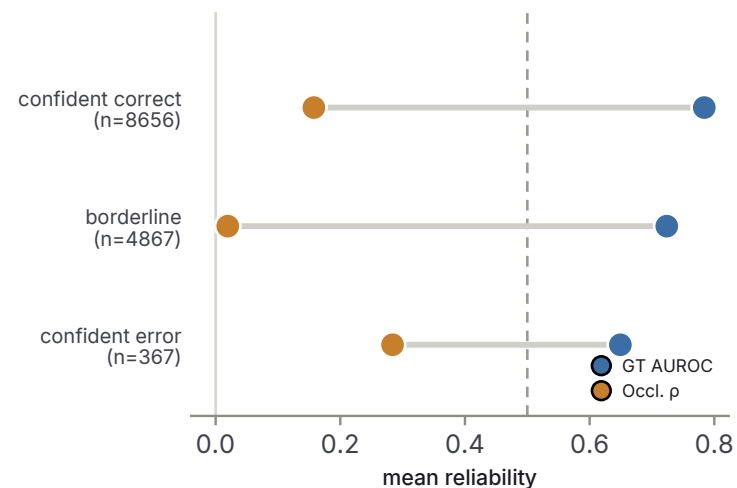
f reliability by regime (pooled)
