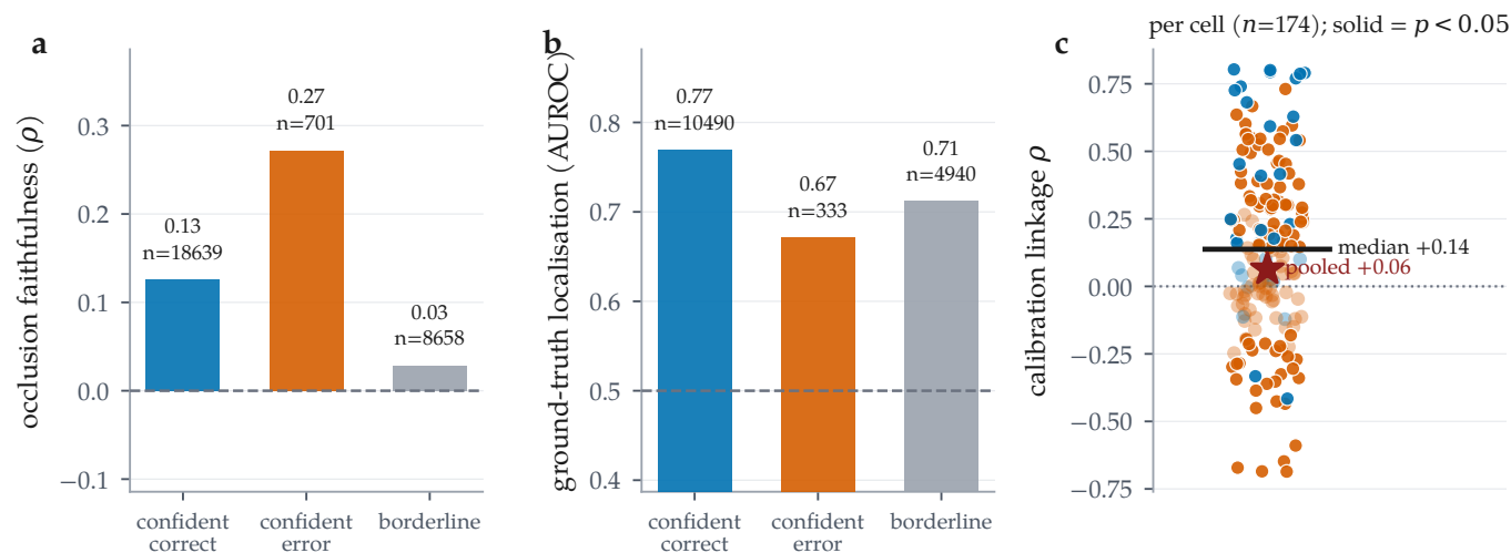
Figure 9: Regime stratification and calibration linkage, over the 31785 per-molecule audit records. (a) Occlusion faithfulness and (b) ground-truth localisation by confidence/correctness regime; n is printed per bar because ground truth exists for only a minority of molecules. Localisation on confident-error molecules degrades (0.769 to 0.671, n = 333 ) while occlusion faithfulness on the same molecules improves (0.126 to 0.272). (c) Calibration linkage computed per cell (solid = p < 0.05 ): the median cell is clearly positive, but pooling all molecules into one correlation attenuates it to near zero, a Simpson’s paradox and a caution against reporting the pooled number.
