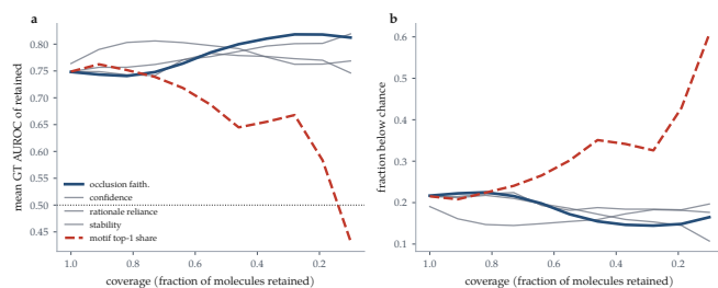
Figure 7: Coverage-reliability curves for abstention signals, over the 15,350 audited molecules that carry ground truth. Every signal is computable at inference time without rationale labels. Moving left to right is abstaining on more molecules. (a) Mean ground-truth localisation of the retained set; the dotted line is chance. (b) The fraction of the retained set whose attribution is below chance — the quantity a deployment is hurt by, and the one the pooled mean in (a) hides. The best signal (occlusion faithfulness) is highlighted; motif top-1 share is dashed because its lift is negative, so abstaining by it makes the retained set worse.
