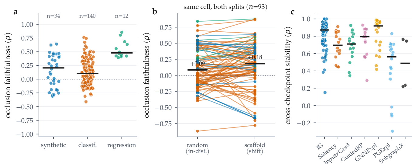
Figure 8: Distributions across all audited combinations. (a) Occlusion faithfulness by dataset regime; bars are medians. (b) The same cell on both splits, joined: faithfulness falls under the scaffold split in only 37 of 93 cells (median change 0.054), so shift does not systematically reduce faithfulness. (c) Cross-checkpoint stability by attributor; the mask-learning methods are not uniformly more stable than the gradient ones.
