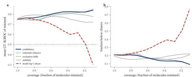
Figure 8: Coverage-reliability curves for abstention signals, over the 10,822 audited molecules that carry ground truth. Every signal is computable at inference time without rationale labels. Moving left to right is abstaining on more molecules. (a) Mean ground-truth localisation of the retained set; the dotted line is chance. (b) The fraction of the retained set whose attribution is below chance — the quantity a deployment is hurt by, and the one the pooled mean in (a) hides. The best signal (predicted confidence) is highlighted; motif top-1 share is dashed because its lift is negative, so abstaining by it makes the retained set worse.
