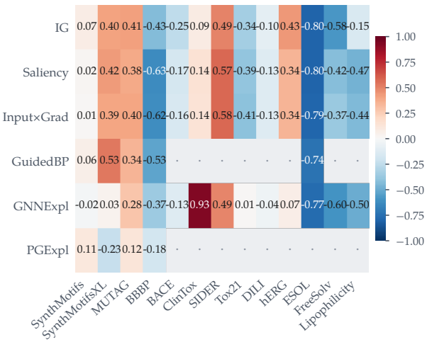
occlusion faithfulness (Spearman \rho )
