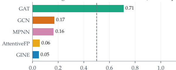
MUTAG · Integrated Gradients · in-distribution (random split)
