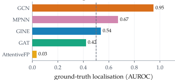
MUTAG · Integrated Gradients · scaffold shift
