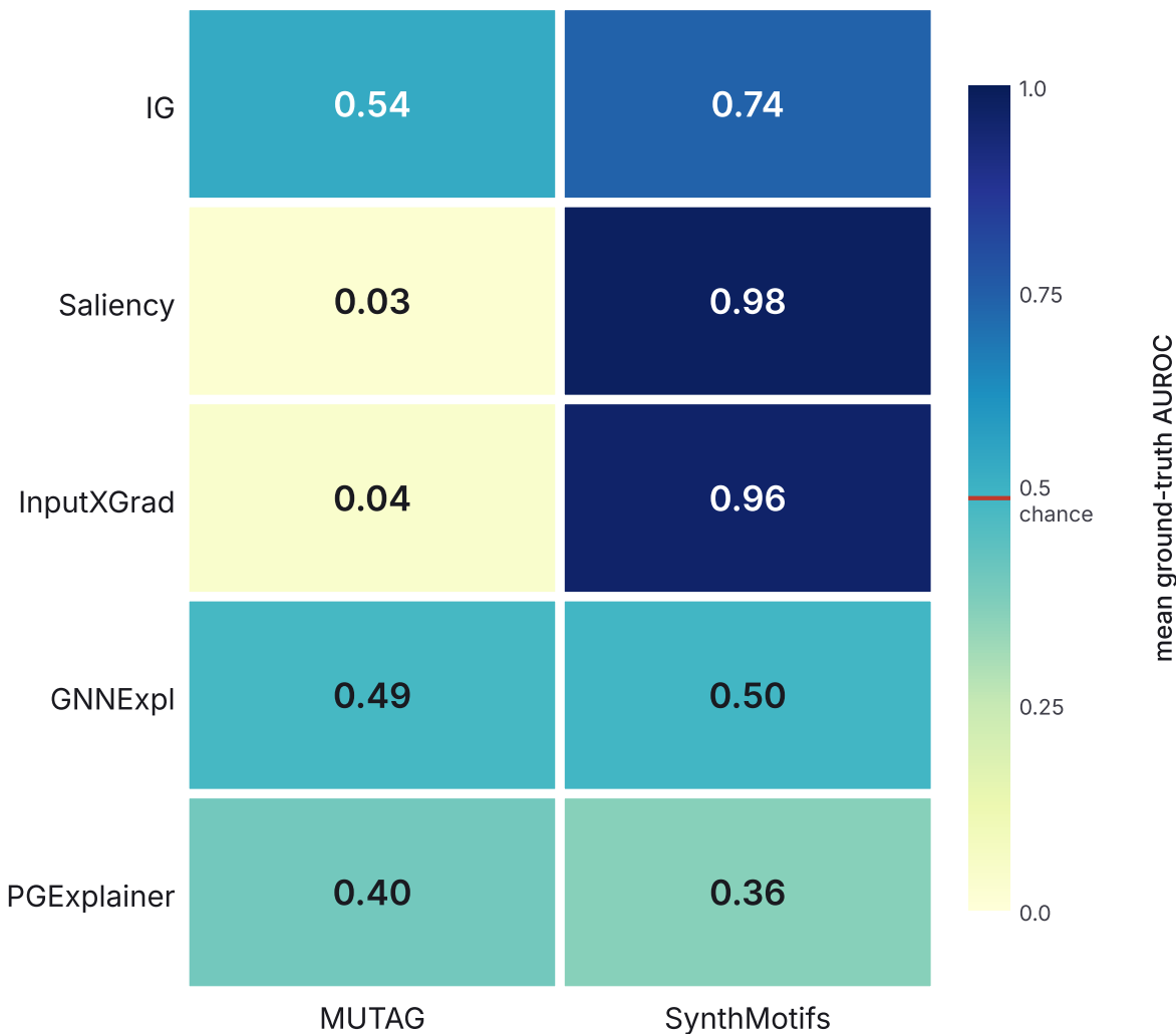
Ground-truth localisation across datasets — GINE
