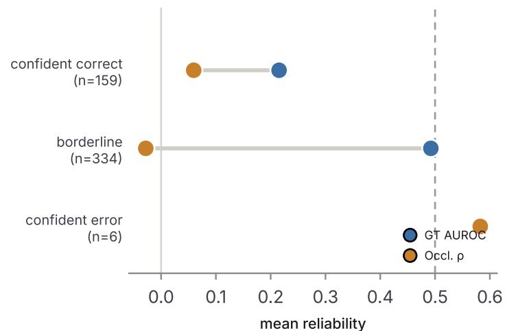
f reliability by regime (pooled)
