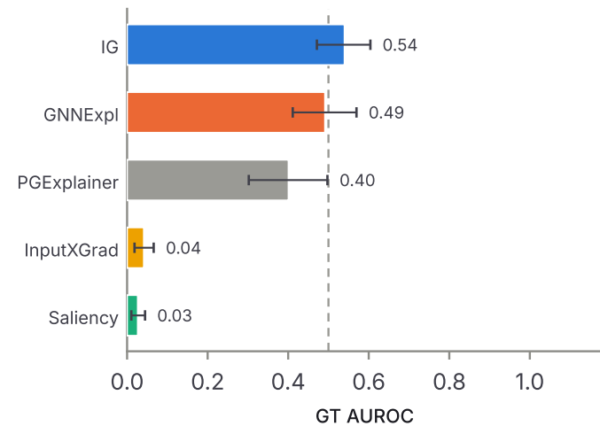
a MUTAG (proxy GT) · by attributor
