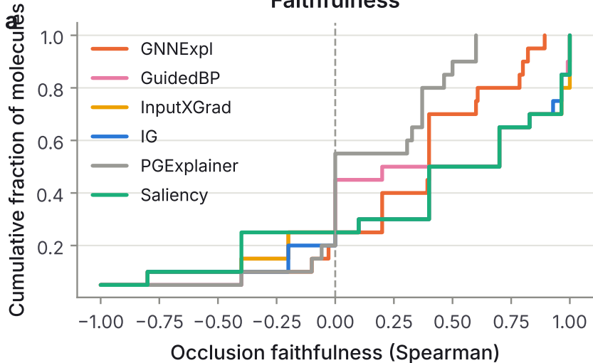
Faithfulness
