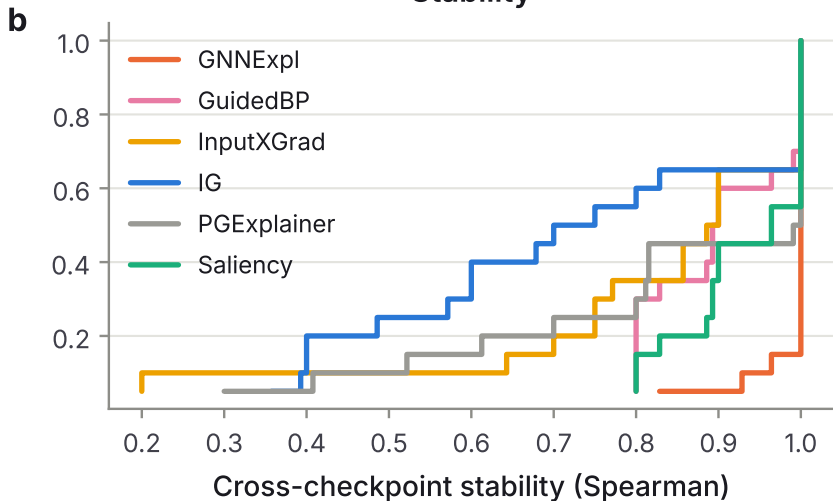
Stability
