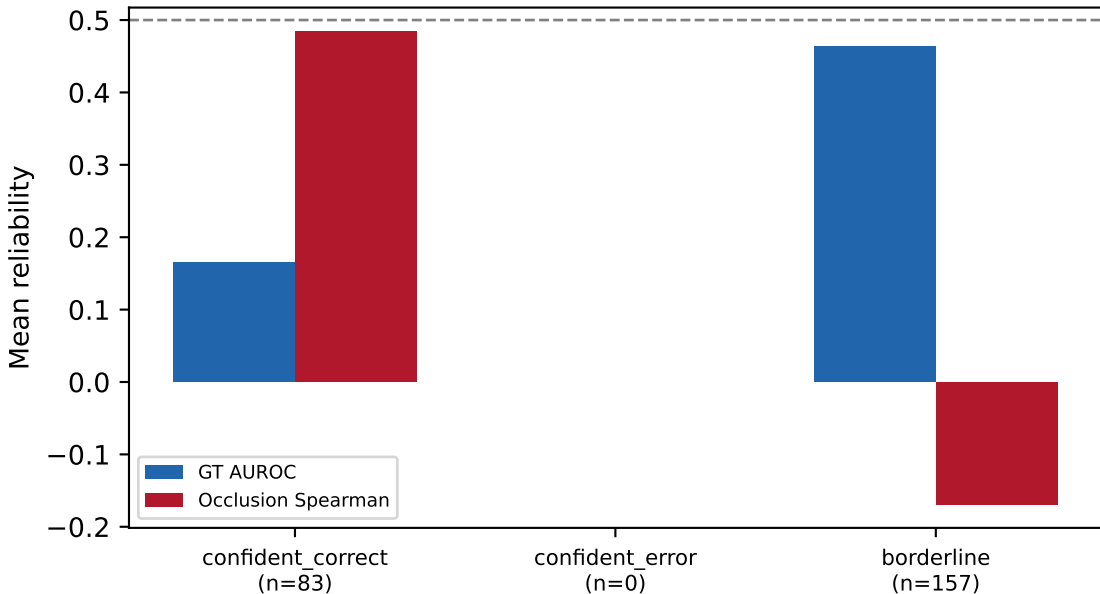
Attribution reliability by regime (scaffold split, pooled)
