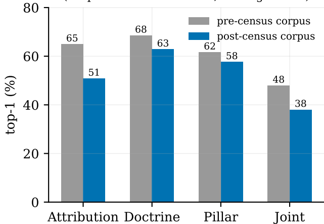
engine accuracy before/after the audit (drop = de-circularization, not regression)
