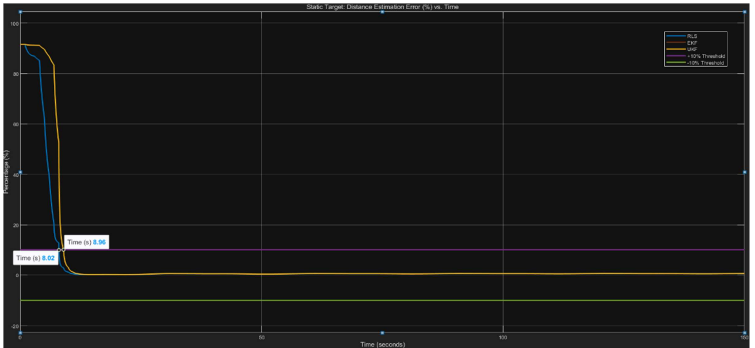
Figure 15: Distance estimation error (%) vs. Time comparison for RLS and UKF/EKF (Static Scenario)
