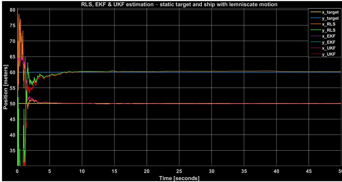
Figure 7: Position tracking comparison for RLS, EKF, and UKF in Scenario A (Static Target)
