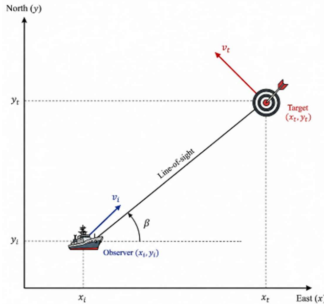
Figure 2: Geometry of the two-dimensional bearing-only tracking model
