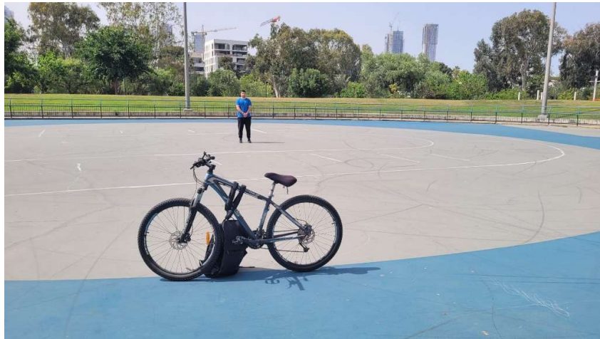
Figure 11: Field testing environment (roller skating rink) and observer platform (bicycle)
