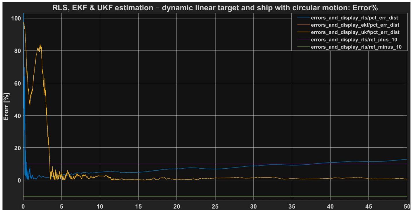
Figure 10: Distance estimation error (%) vs. Time comparison for RLS, EKF, and UKF in Scenario B (Dynamic Target)
