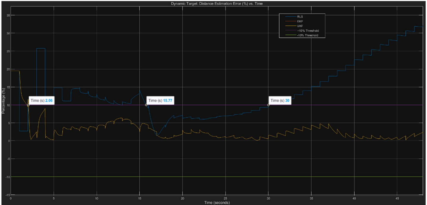
Figure 18: Distance estimation error (%) vs. Time comparison for RLS and UKF/EKF (Dynamic Scenario)
