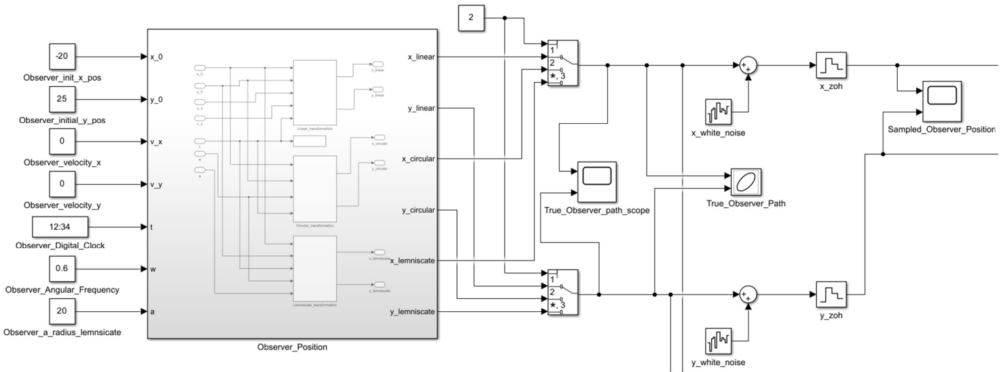
Figure 3: Simulink block diagram of the Coordinate Generation subsystem
