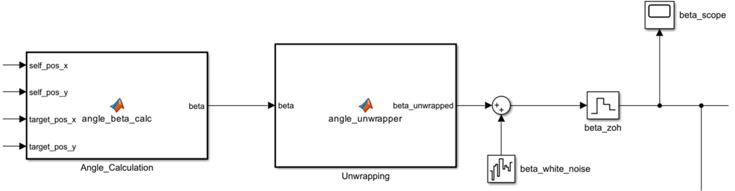
Figure 4 : Simulink block diagram for relative bearing calculation and signal unwrapping
