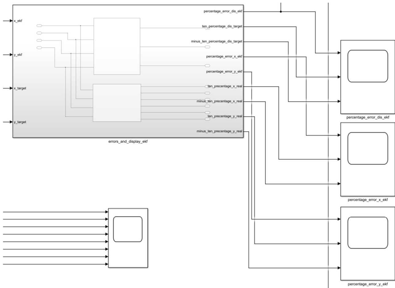
Figure 6: Simulink block diagram of the error calculation subsystem
