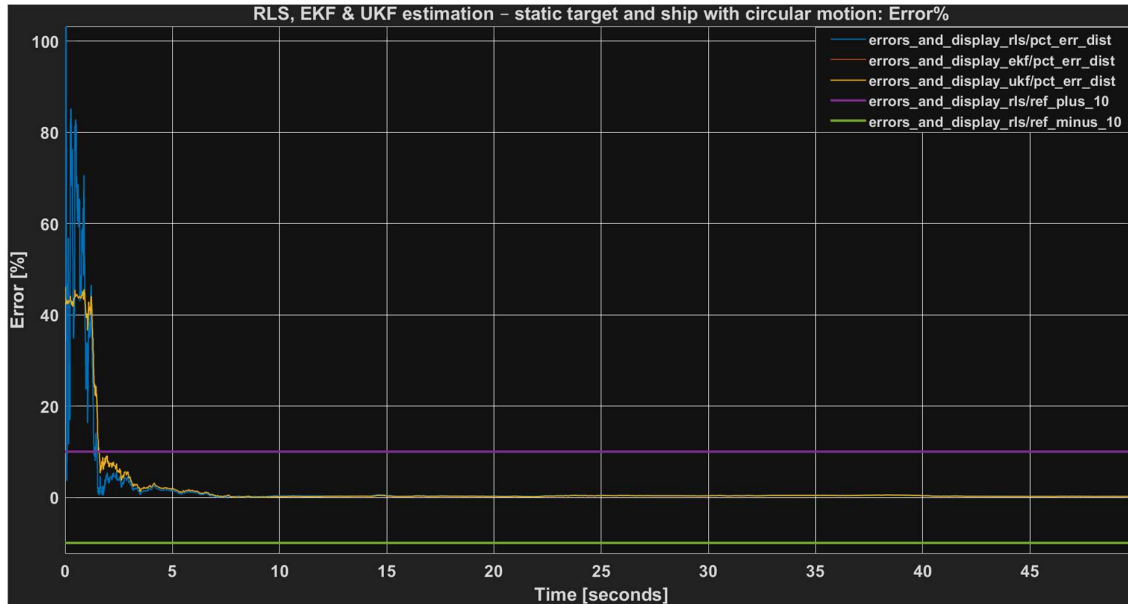
Figure 8: Distance estimation error (%) vs. Time comparison for RLS, EKF, and UKF in Scenario A (Static Target)
