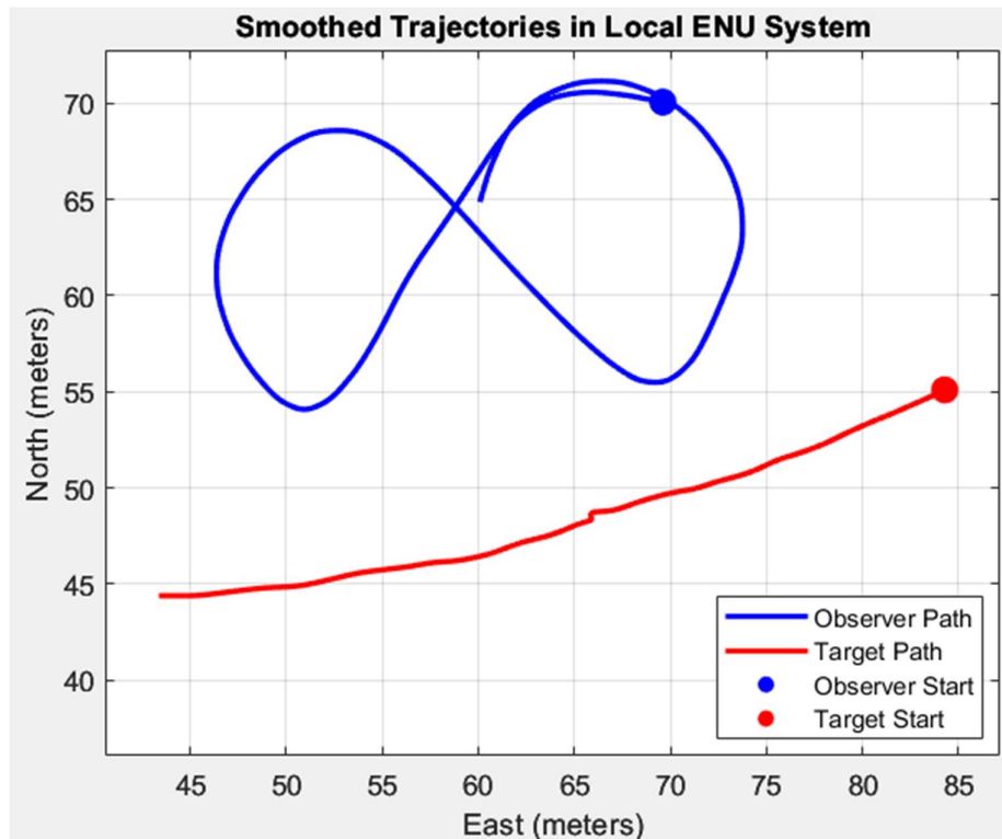
Figure 16: Figure-eight observer path and linear target path in local ENU system (Dynamic Scenario)
