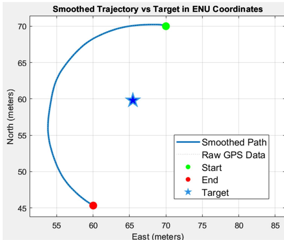
Figure 13: Smoothed observer path and true target coordinates in ENU system (Static Scenario)
