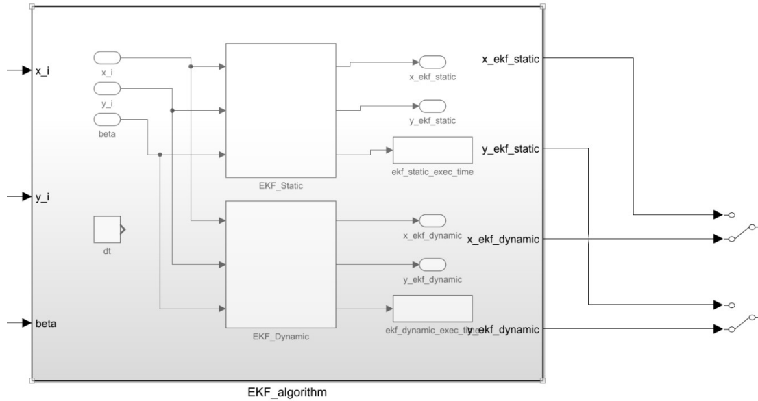
Figure 5: Simulink EKF Algorithm architecture
