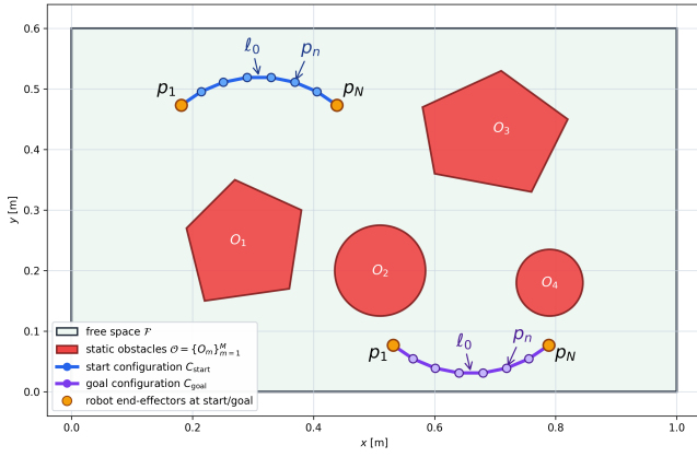
Figure 1: Problem formulation for global cable routing in a planar workspace with static obstacles.
