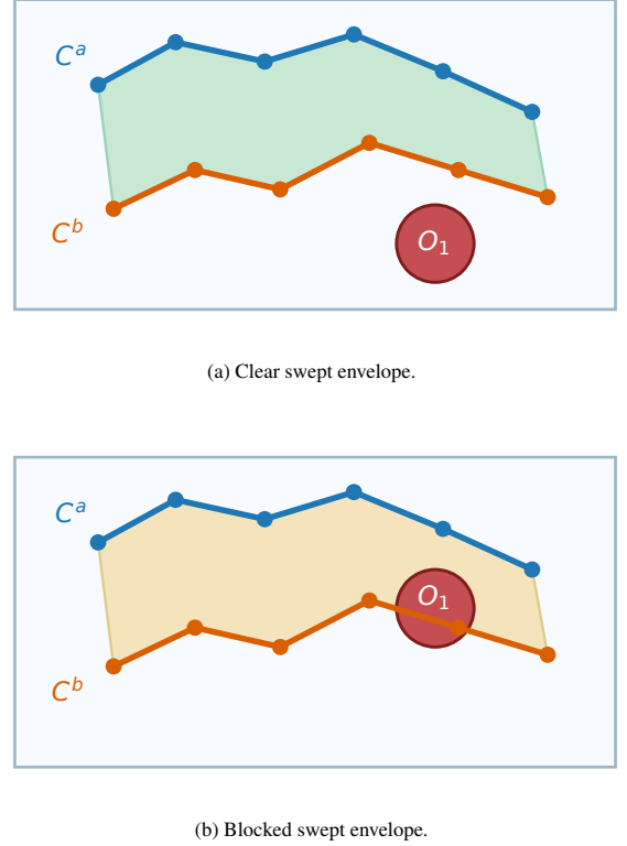
Figure 5: Transition feasibility between two ordered configurations. Blue and orange curves denote the two neighboring cable shapes, the shaded band is the swept envelope, and red regions denote obstacles. The complete edge is accepted only when the swept region is obstacle-free and the remaining conditions in \Gamma(\cdot, \cdot) are also satisfied.
