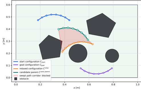
(b) Rejected parent connection. The swept corridor intersects an obstacle, so the transition from the candidate parent to the ordered relaxed configuration is not sweep-clear.
