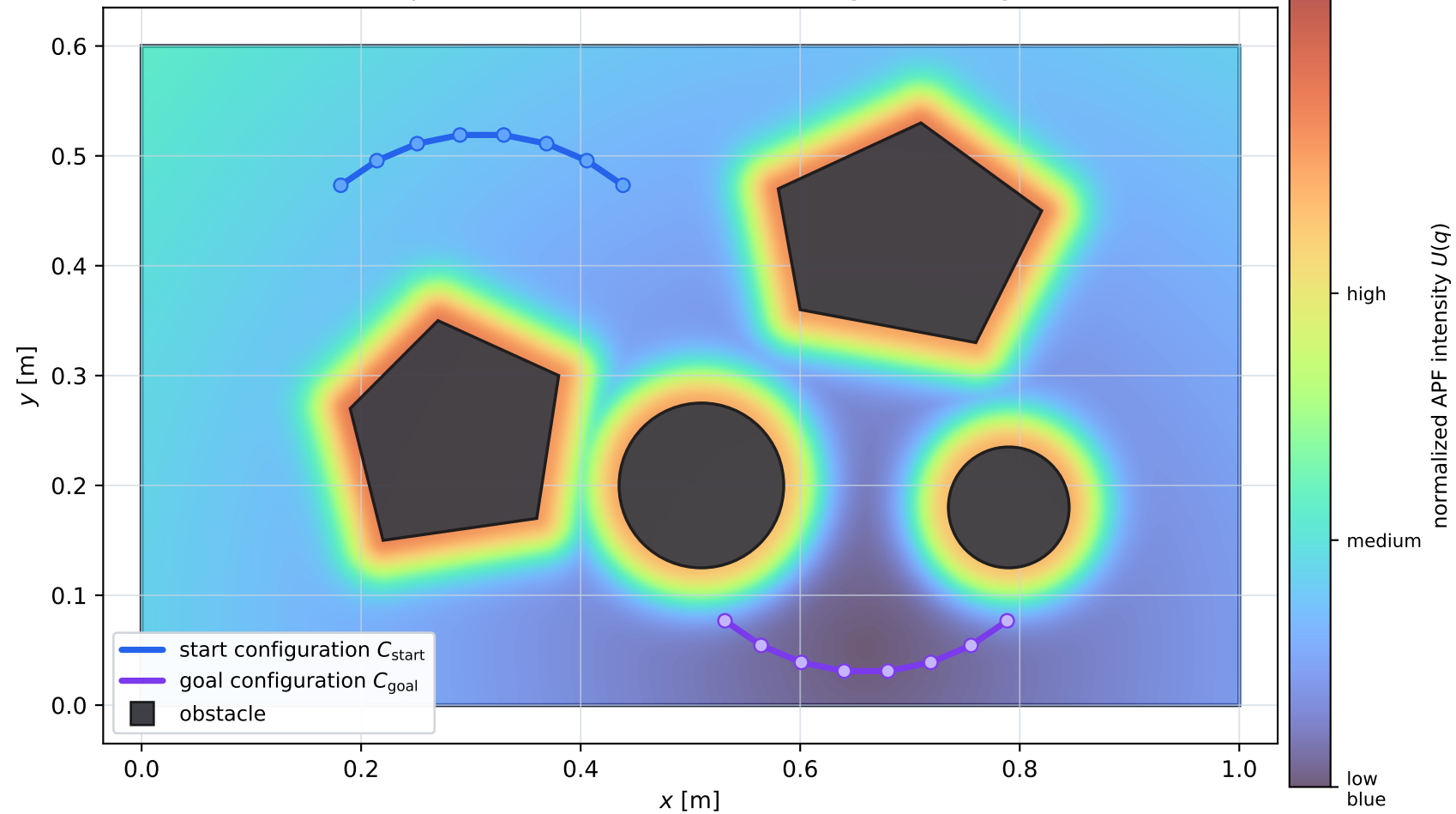
start-tree potential field: attraction to goal configuration
