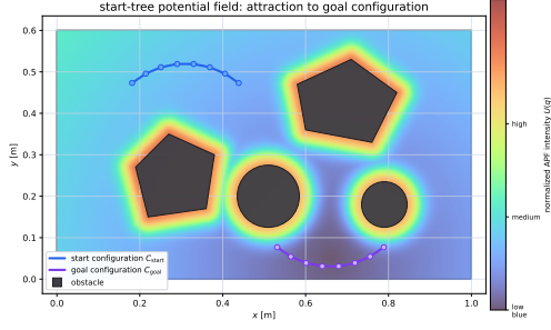
(a) Start-tree APF with attraction toward the goal configuration.
