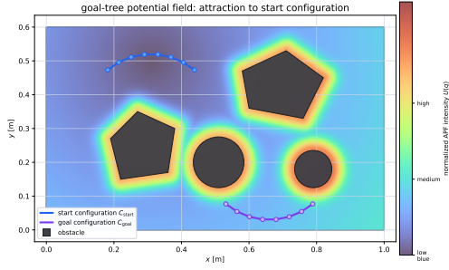
(b) Goal-tree APF with attraction toward the start configuration.
