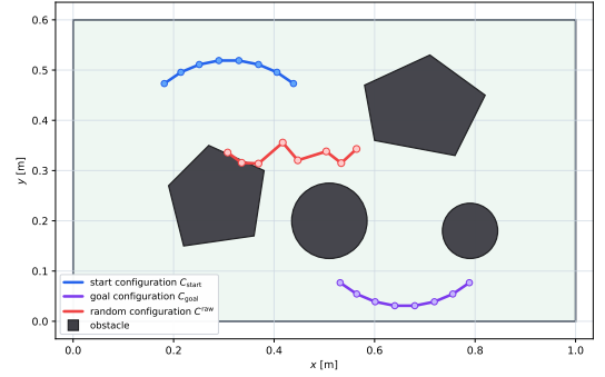
(a) Sampled raw configuration C^{\text{raw}} .
