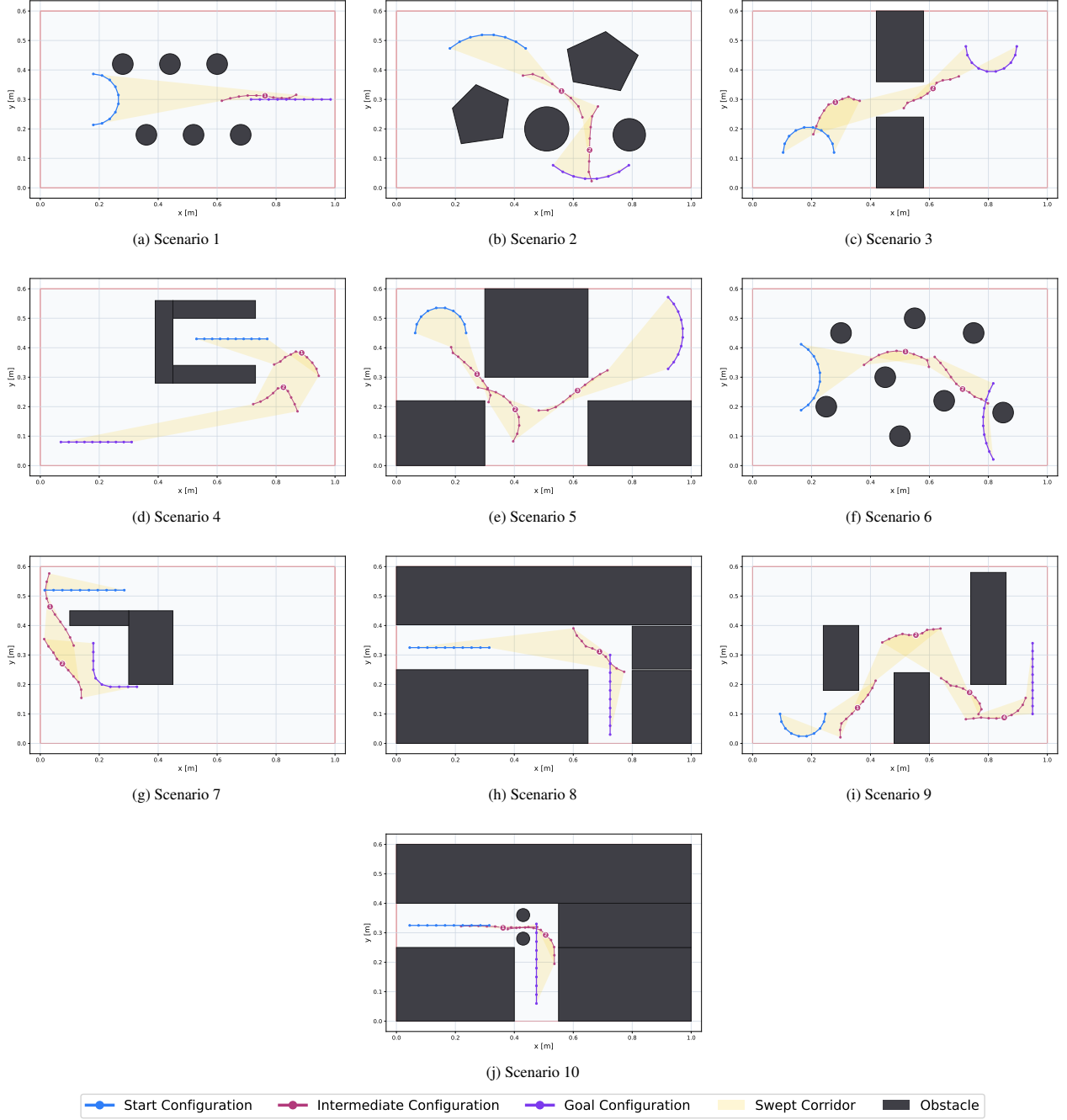
Figure 12: Representative GCR solutions for the ten benchmark scenarios. Each subfigure shows the initial cable configuration, the target cable configuration, the static obstacles, and the resulting deformation sequence.
