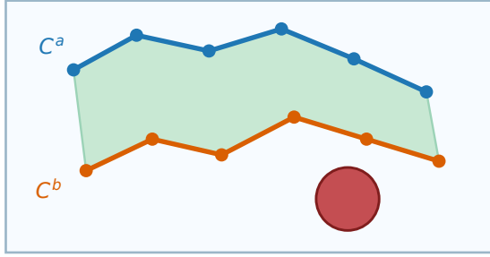
(a) Clear swept envelope.
