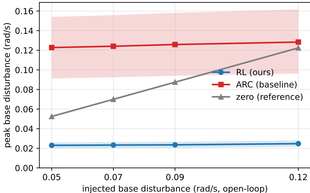
Base-attitude disturbance rejection
