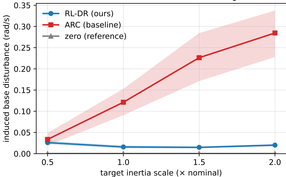
Induced base-attitude disturbance vs target inertia
