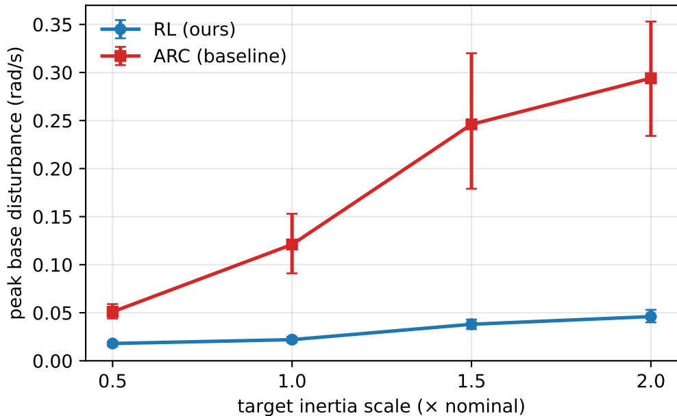
Inertia parity (no injected disturbance)
