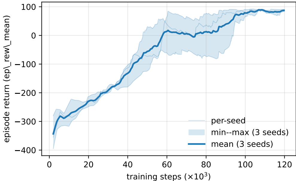
Training: detumbling policy (SAC, base-disturbance DR)
