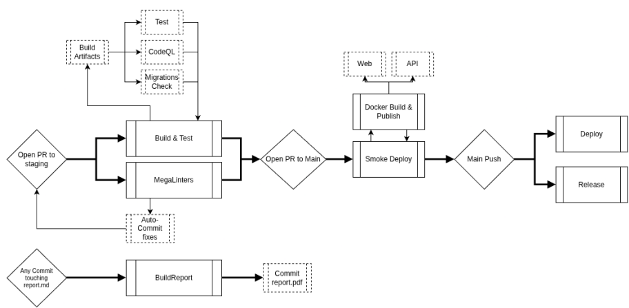
Figure 3: DevOps CICD.png
