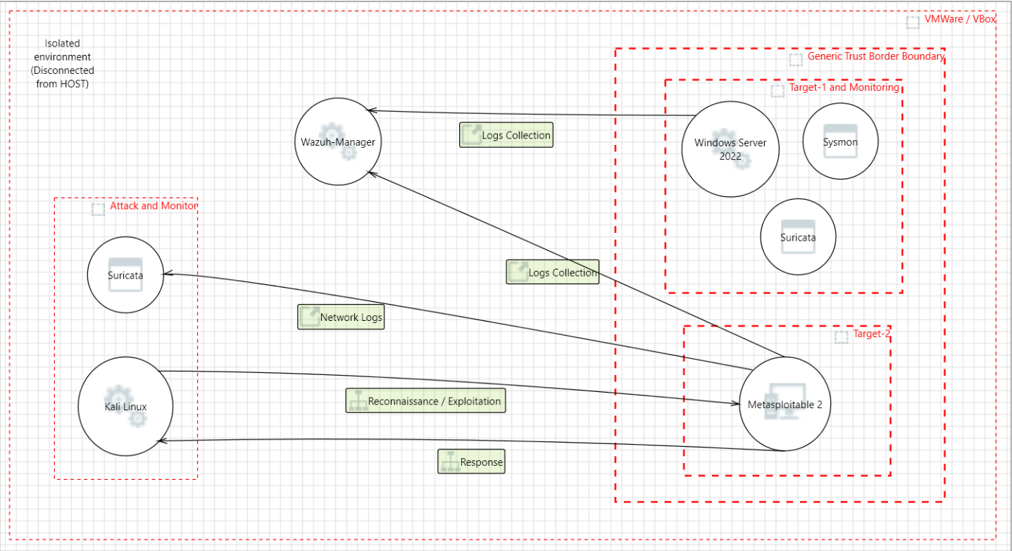
Figure 9: Threat Modeling on Microsoft Threat Modeling Tool
