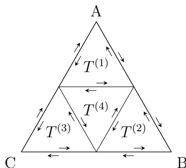
Figure 1: Splitting the integral \eta(T) .
