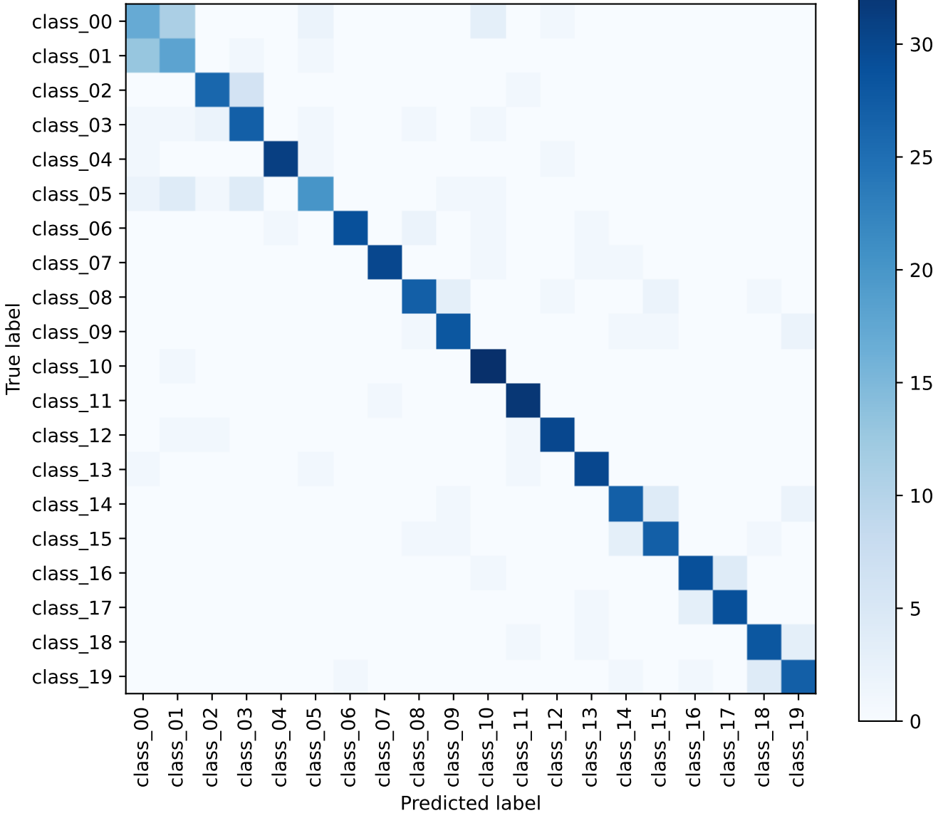
Test confusion matrix (average per-class accuracy = 0.815)
