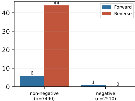
Errors by sign of the answer
