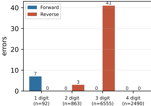
Errors by answer length
