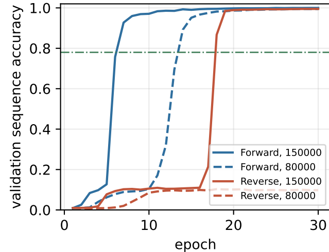
Convergence by direction and data size
