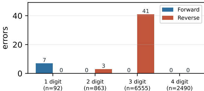
Errors by answer length
