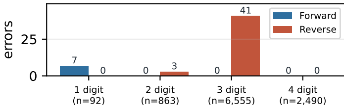
Errors by answer length
