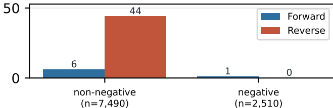
Errors by sign of the answer
