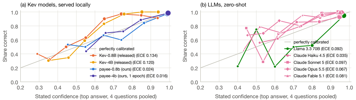
Fig. 3. Reliability on the test split: share of answers correct against stated confidence, in 10 bins over the four questions pooled. Marker area grows with the answers in a bin; bins with fewer than 10 are omitted.
