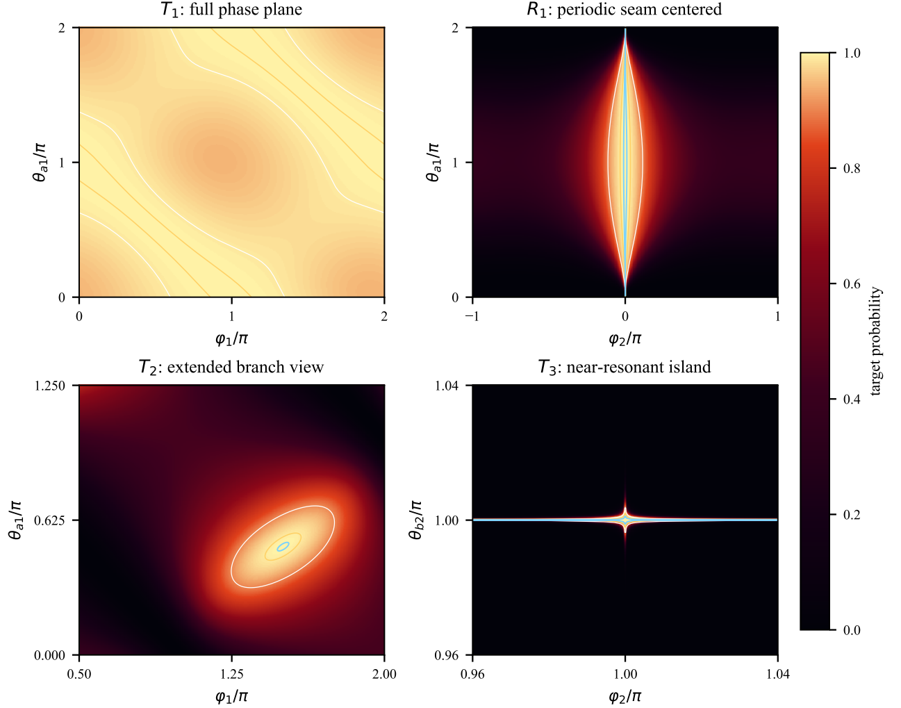
FIG. 2. Representative phase-coordinate routing landscapes for four fixed-backbone routing mechanisms under waveguide-1 edge incidence. The T_1 panel shows the full 0-2\pi phase plane, while the R_1 panel is recentered at the periodic seam so that the two edge features join into one continuous high-transmission region. The T_2 panel uses an extended branch window large enough to show the boundary of the high-fidelity island around the correlated branch neighborhood introduced below. The T_3 panel uses a magnified near-resonant window because the far-waveguide high-fidelity region is much narrower on the full phase torus. Contours mark P = 0.9, 0.99 , and 0.999 where visible. These two-dimensional cuts demonstrate sufficient high-probability routes around representative optima; they are not intended as uniqueness proofs for the corresponding routing conditions. The complete six-target optimized parameter record is given in Table III; the symmetry-related R_2 and R_3 maps are retained in the repository all-target figure.
