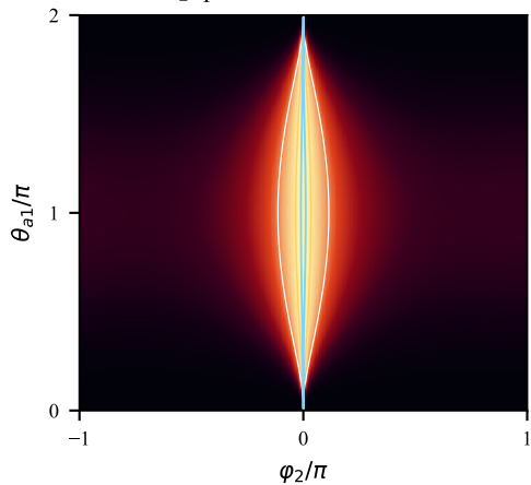
T_3 : near-resonant island
