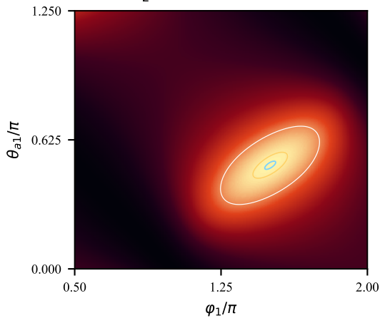
T_2 : extended branch view
