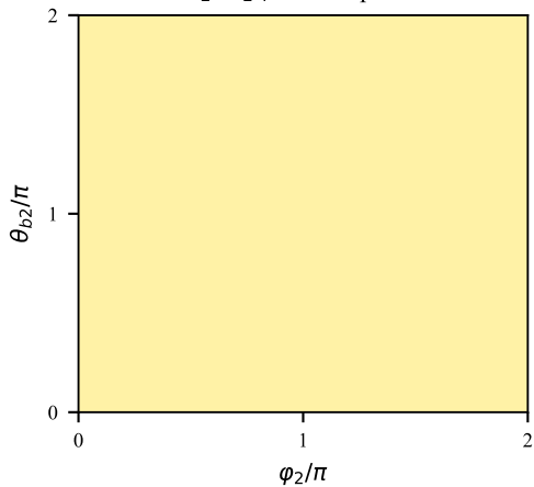
T_2 : extended branch view
