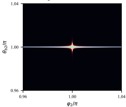
T_3 : near-resonant island
