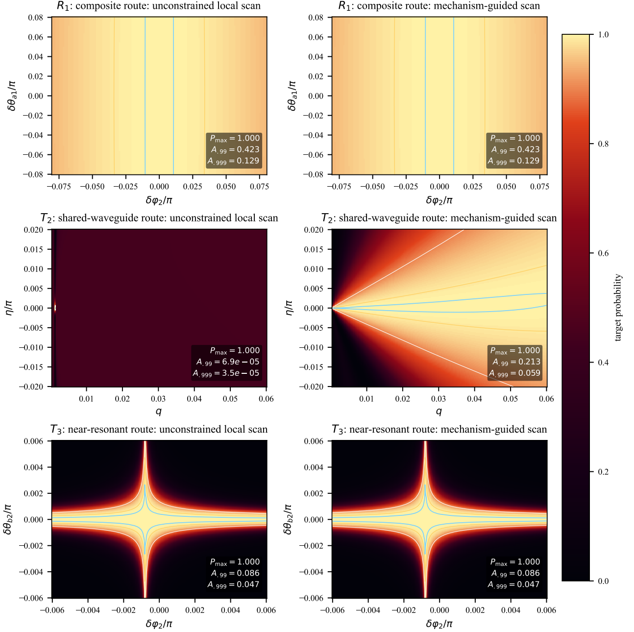
FIG. 3. Representative mechanism comparison for nontrivial waveguide-1 edge-incidence routes. Rows show R_1 (same-waveguide composite reflection), T_2 (shared-waveguide routing), and T_3 (near-resonant far-waveguide routing). Left column: unconstrained local two-parameter scans around the optimized point. Right column: mechanism-guided scans. The T_2 row imposes the analytic correlated branch \mathcal{C}_2(q) defined in Eq. (24). The R_1 row uses direct-oracle numerical continuation of \theta_{a1} around the optimized composite route, and the T_3 row uses direct-oracle detuning-guided continuation around the near-resonant route; no analytic R_1 or T_3 branch is assumed. All panels use the same probability color scale; contours mark P = 0.9, 0.99 , and 0.999 where visible. The displayed area fractions compare the high-fidelity basins for representative mechanisms rather than enumerating all six output channels.
