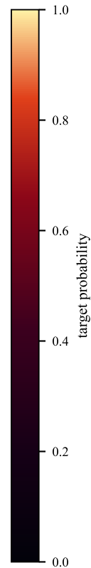
R_3 : near-resonant island
