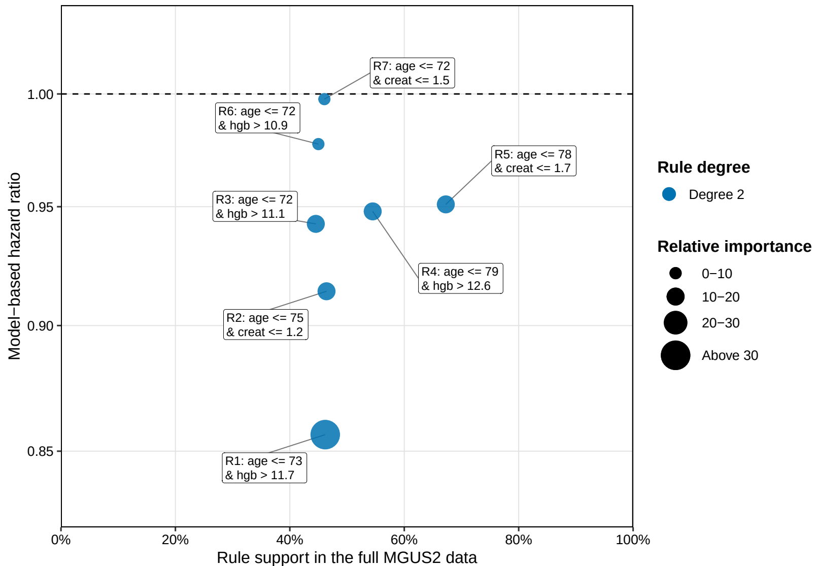
Rule support-effect map of selected BRP-GABLE rules
