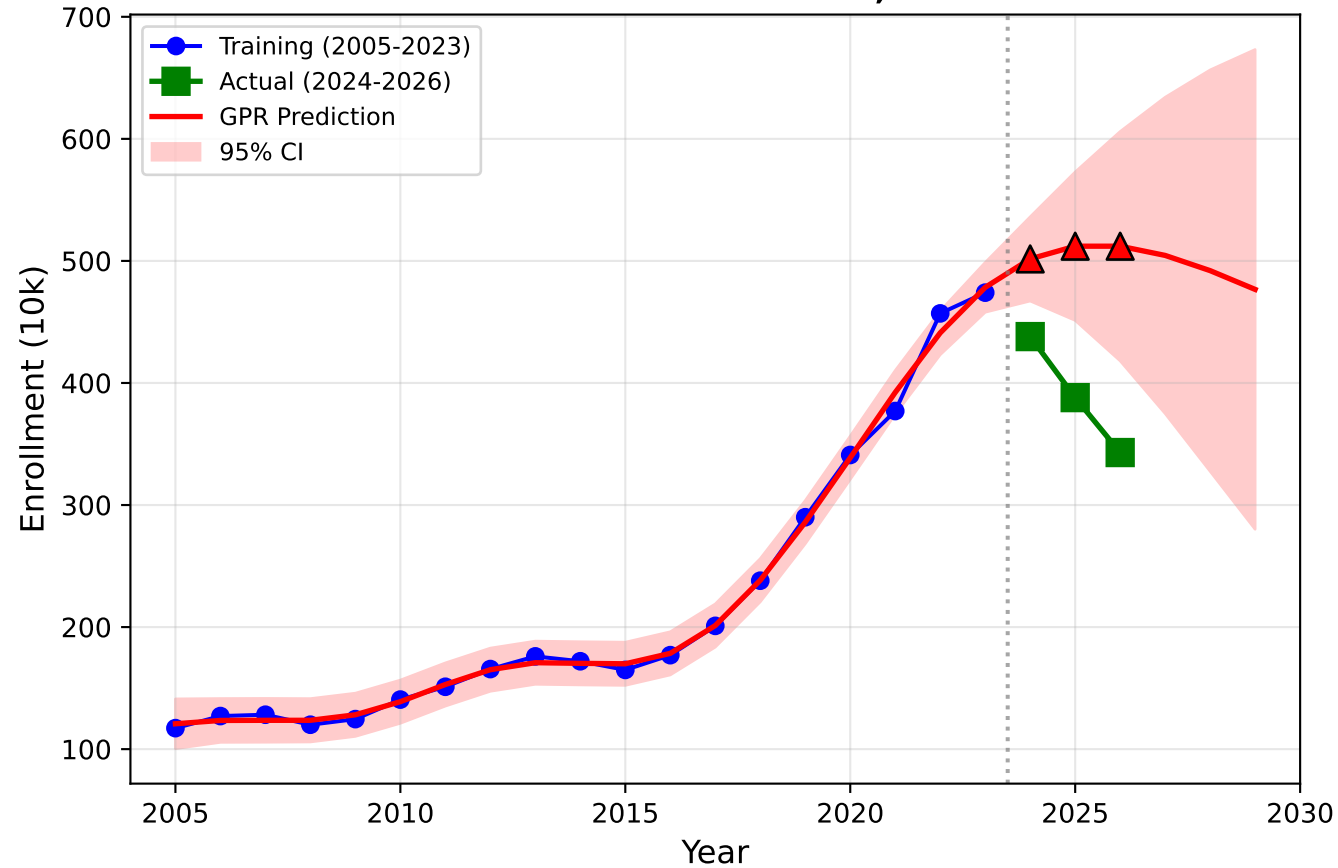
GPR Prediction: RMSE=126.5, MAE=118.9
