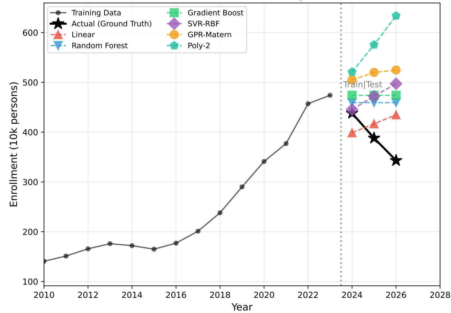
All Models Prediction Comparison
