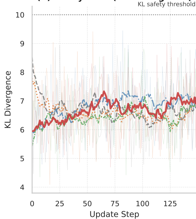
(b) Policy Drift (KL Divergence)
