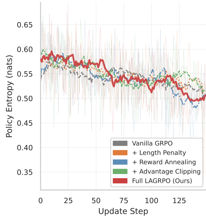
(a) Policy Entropy
