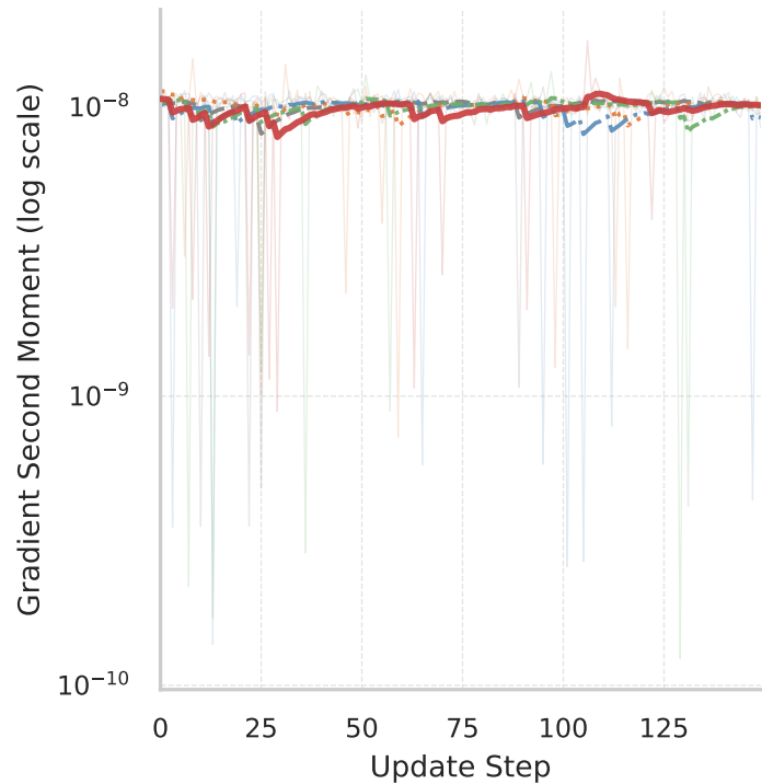
(c) Optimization Variance
