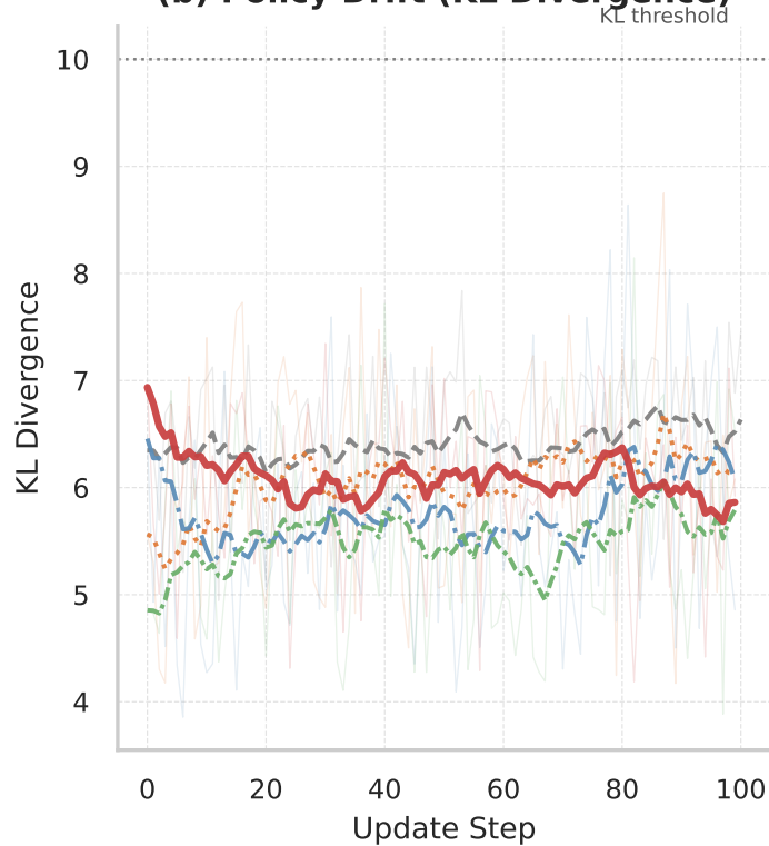
(b) Policy Drift (KL Divergence)
