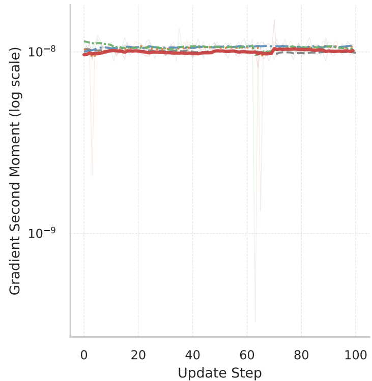
(c) Optimization Variance (Gradient Second Moment)
