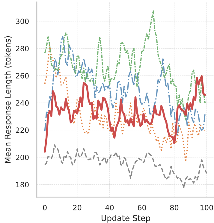
(b) Mean Response Length
