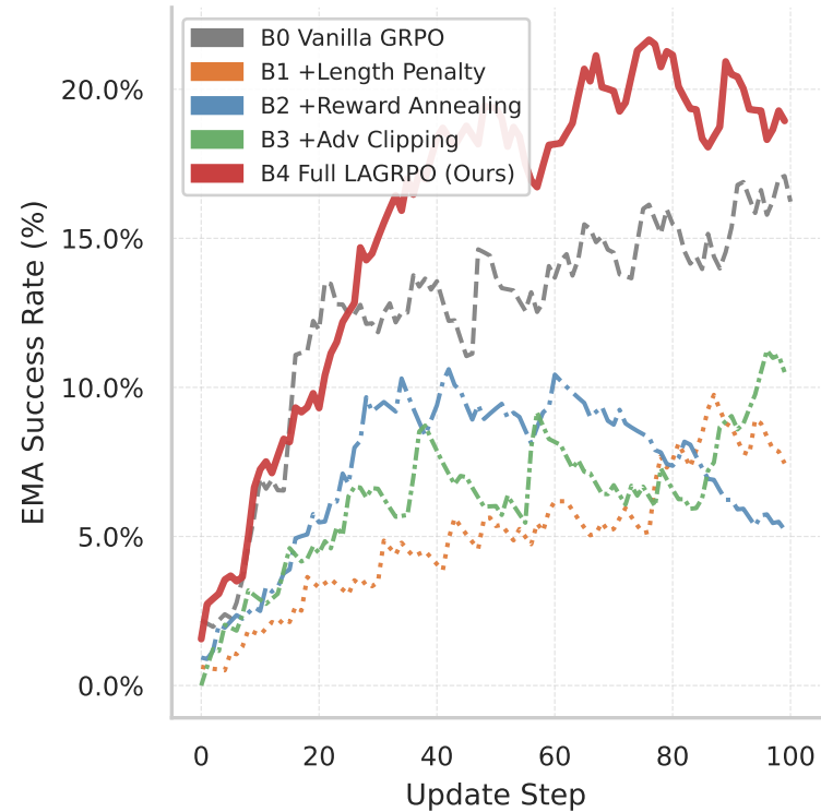
(a) EMA Success Rate
