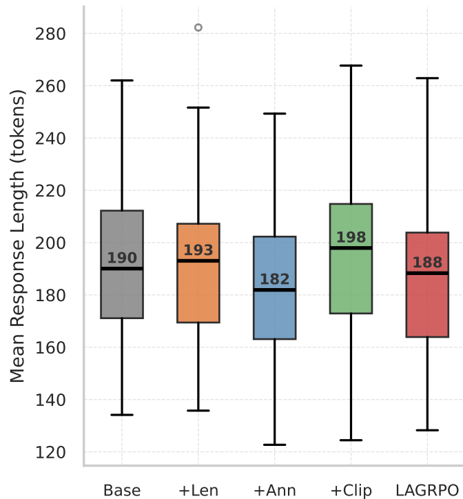
(b) Output Length Distribution
