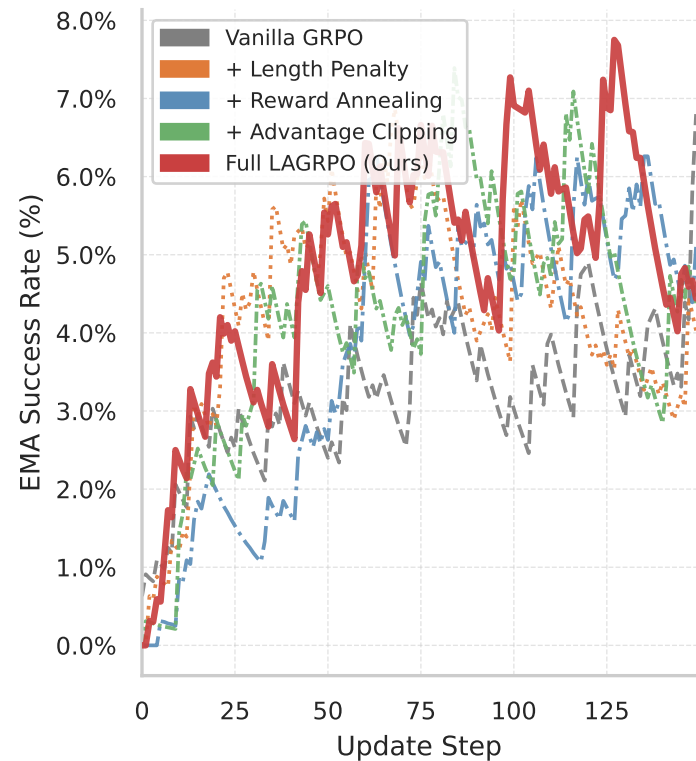
(a) EMA Success Rate
