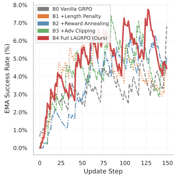
(a) EMA Success Rate (Mixed Difficulty)
