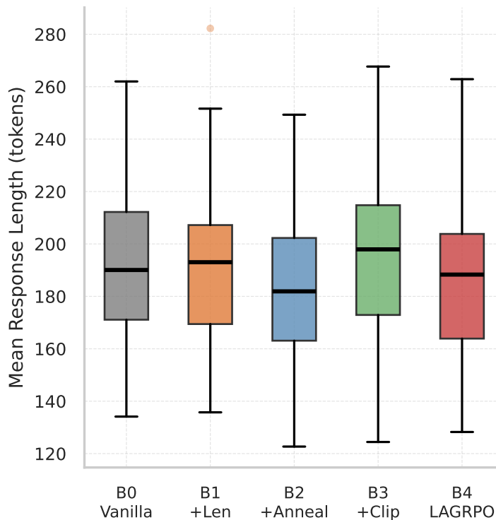
(b) Output Length Distribution
