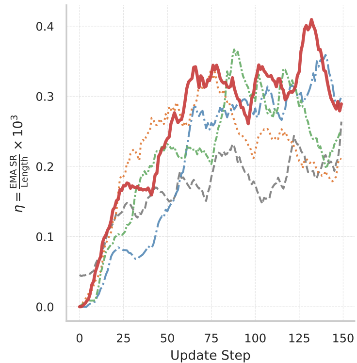
(c) Exploration Efficiency ( \eta )
