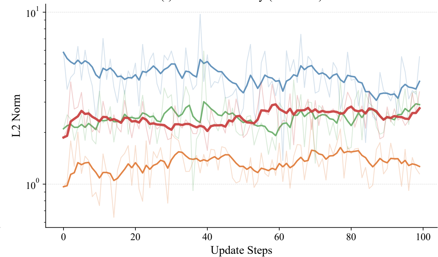
(f) Gradient Stability (L2 Norm)
