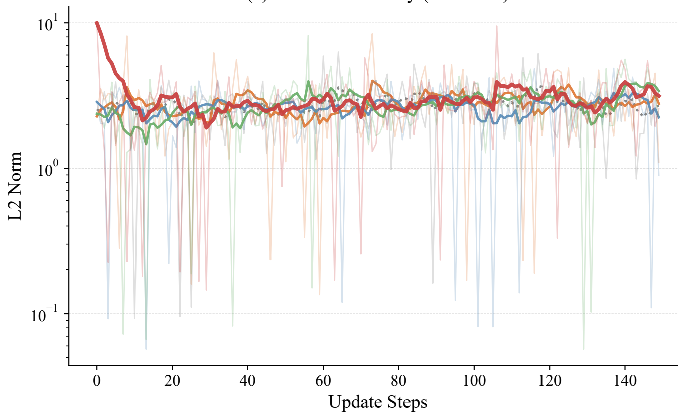
(e) Gradient Stability (L2 Norm)
